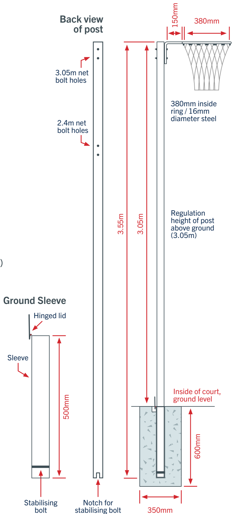
Side view of post
